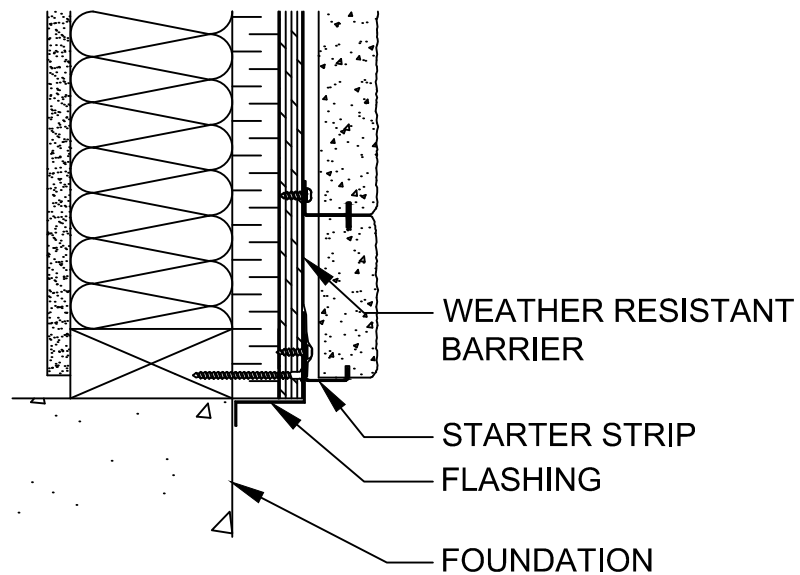
SECTION AT STARTER STRIP
